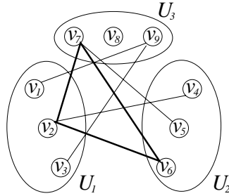
FIG. 2 an instance (G, k = 3, \{U_1 = \{v_1, v_2, v_3\}, U_2 = \{v_4, v_5, v_6\}, U_3 = \{v_7, v_8, v_9\}\}) for PCLIQUE. The vertices \{v_2, v_6, v_7\} form a PCLIQUE of size 3.
